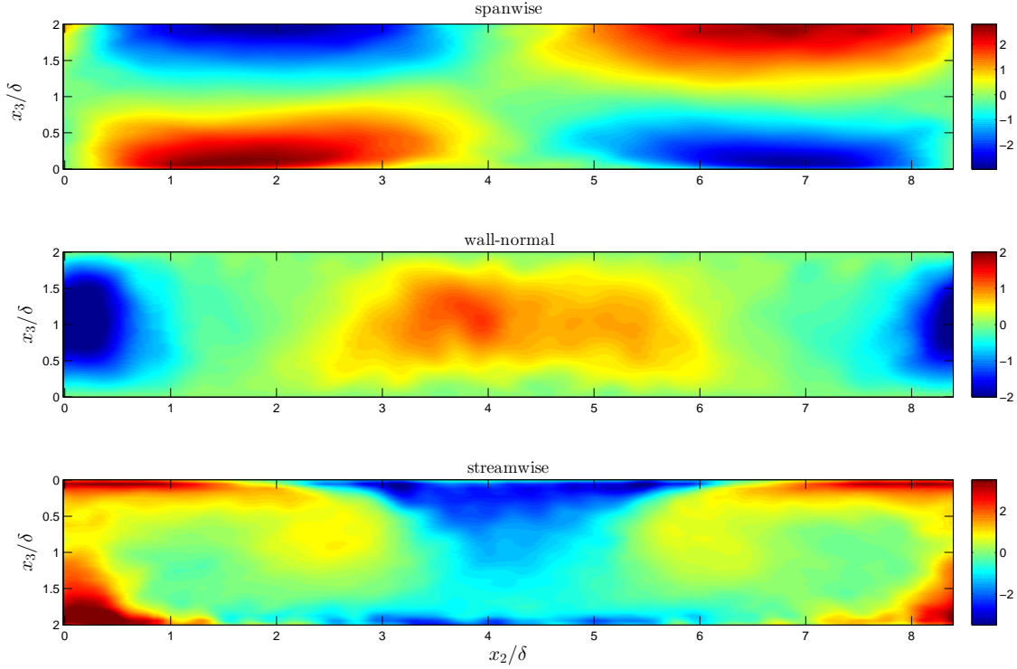
Figure 4.1: Spanwise-vertical variation of streamwise- and time-averaged spanwise (top), wall-normal (middle) and streamwise (bottom) velocity fluctuations defined in Eq. (3.26) from LES-NWM in the domain L_1/\delta \times L_2/\delta \times L_3/\delta = 4\pi \times \frac{8}{3}\pi \times 2 . Results were obtained with the traditional wall model described in sub-section 4.1.1 with B = 6.5 in (4.8). Streamwise (downwind) direction ( x_1 ) is out of page.
